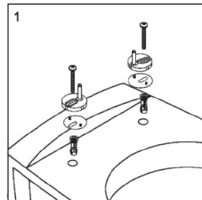
1 Insert the hinges into the toilet.
